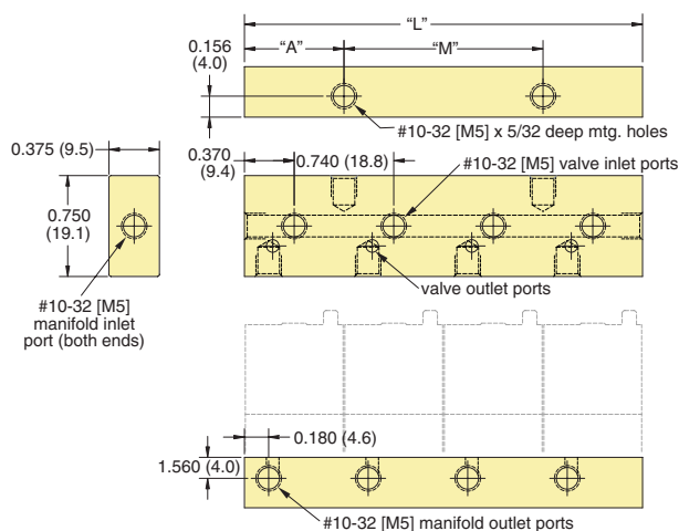
Single-Sided
