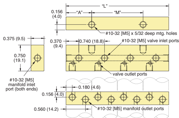
Double-Sided
