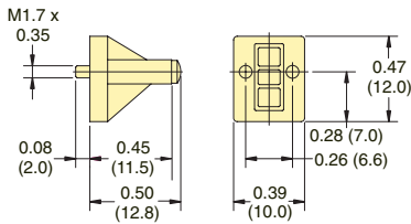
Mounting Interface
