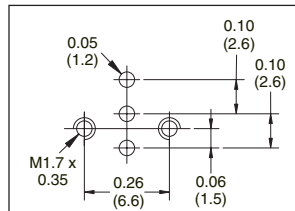
Mounting Interface
