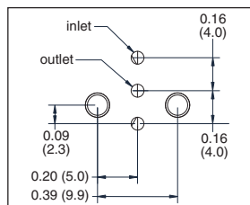
Mounting Interface
