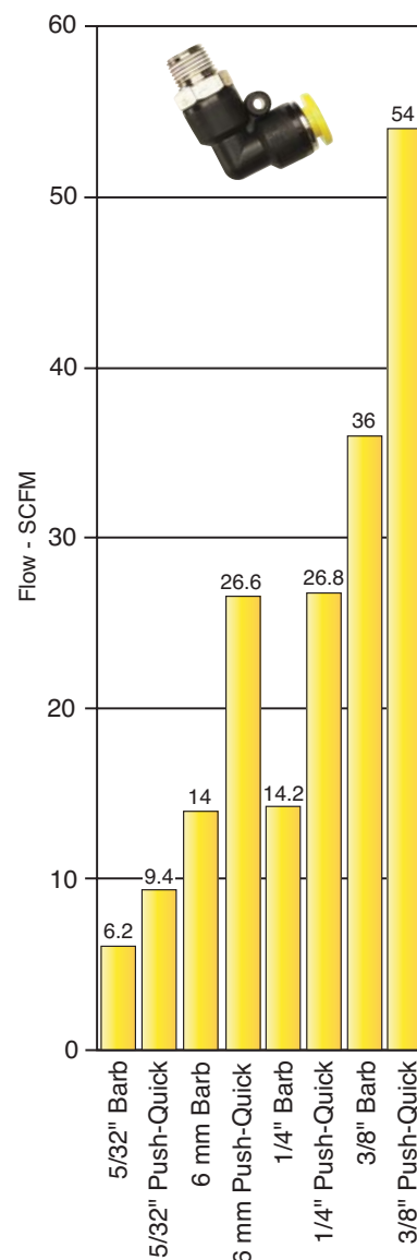
Barb vs Push-Quick Fittings Flow Comparison @ 100 psig
