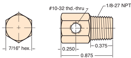
1/8" NPT to #10-32 "X" Cross Fitting
