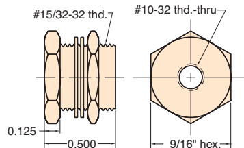
#10-32 Bulkhead Fitting
