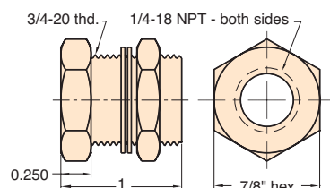
1/4" NPT Bulkhead Fitting
