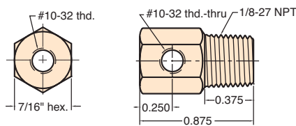
#10-32 Bulkhead Fitting
